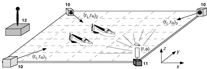
Figure 2. Sensing of shoe position
